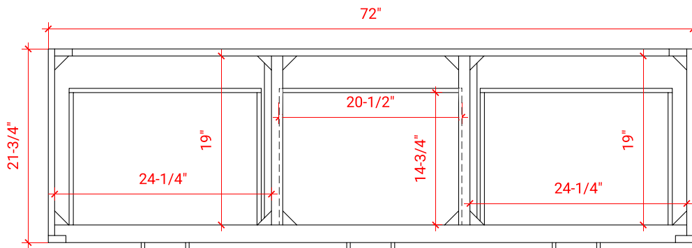
PLAN VIEW
