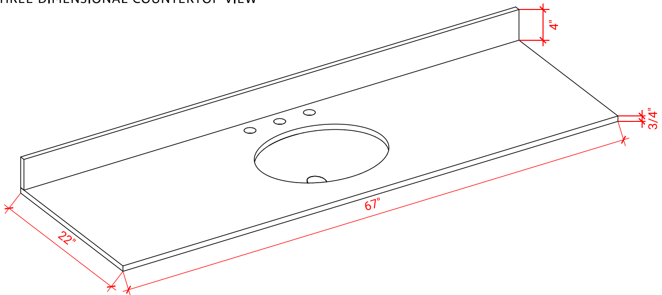
THREE DIMENSIONAL COUNTERTOP VIEW
