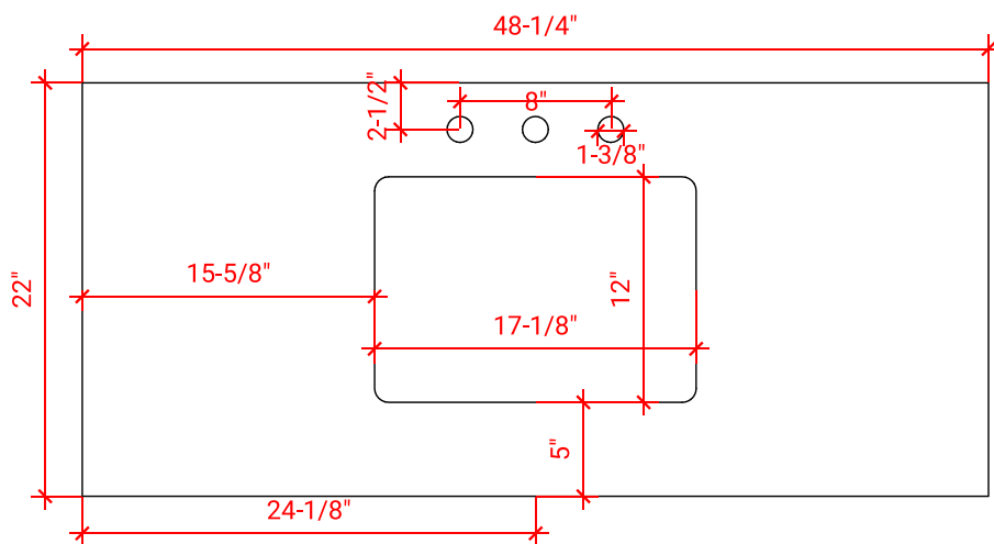
COUNTERTOP PLAN VIEW
